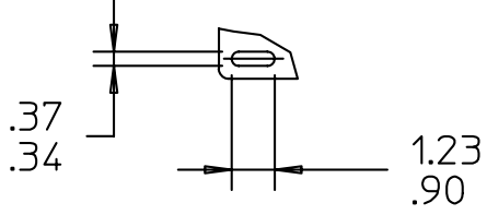
SLOT DETAIL (TYP. 4)
