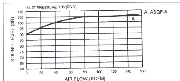
ASQF-8 dB Rating vs. Air Flow
